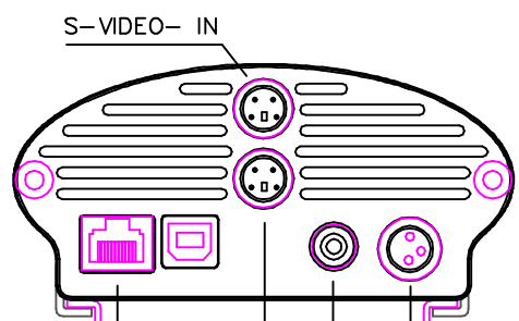
REAR OF CAMERA SHOWING INTERFACE OPTIONS
